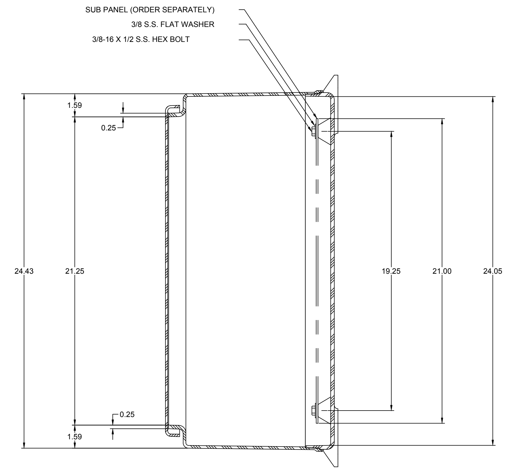
SECTION B-B
