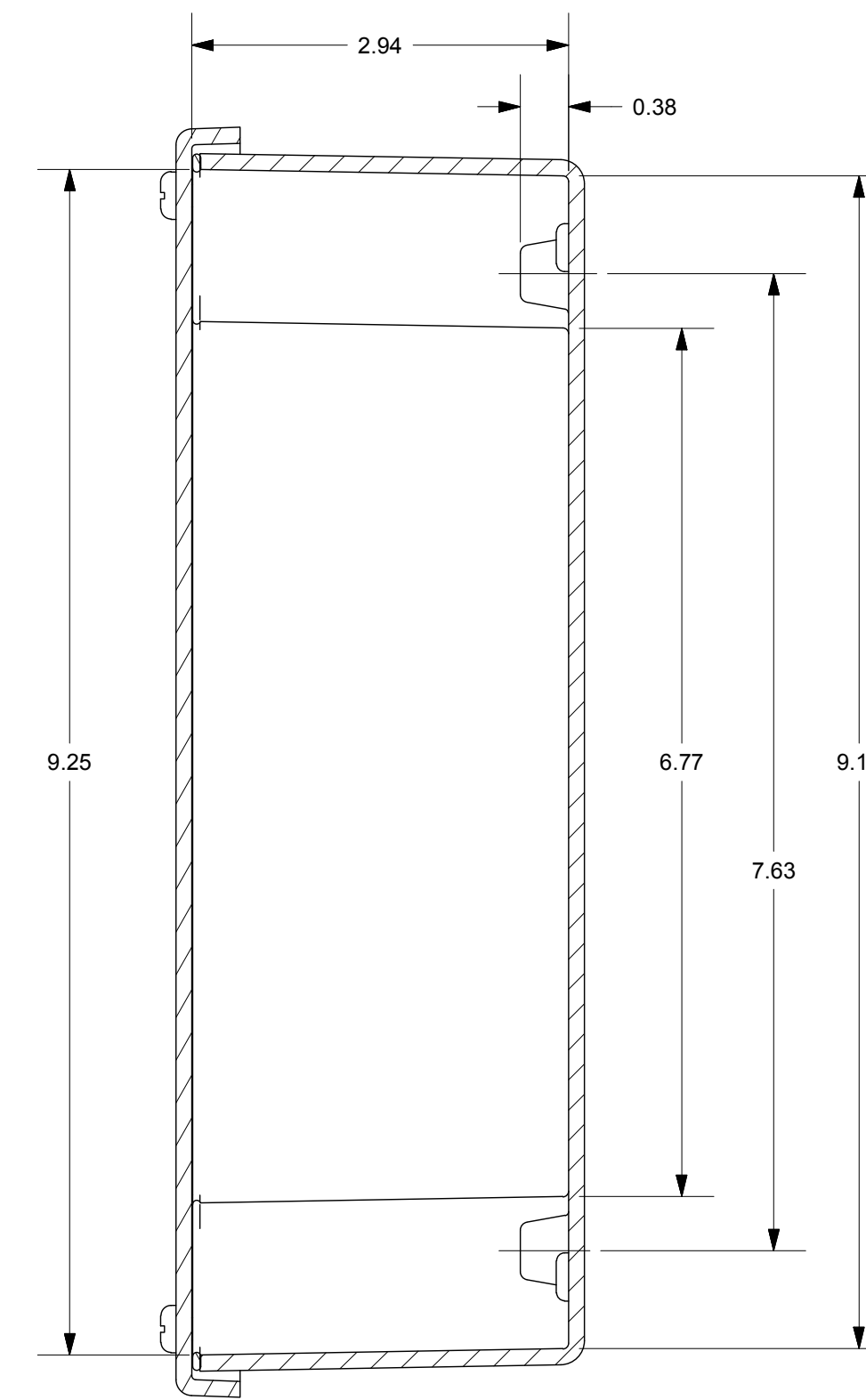
SECTION B-B
