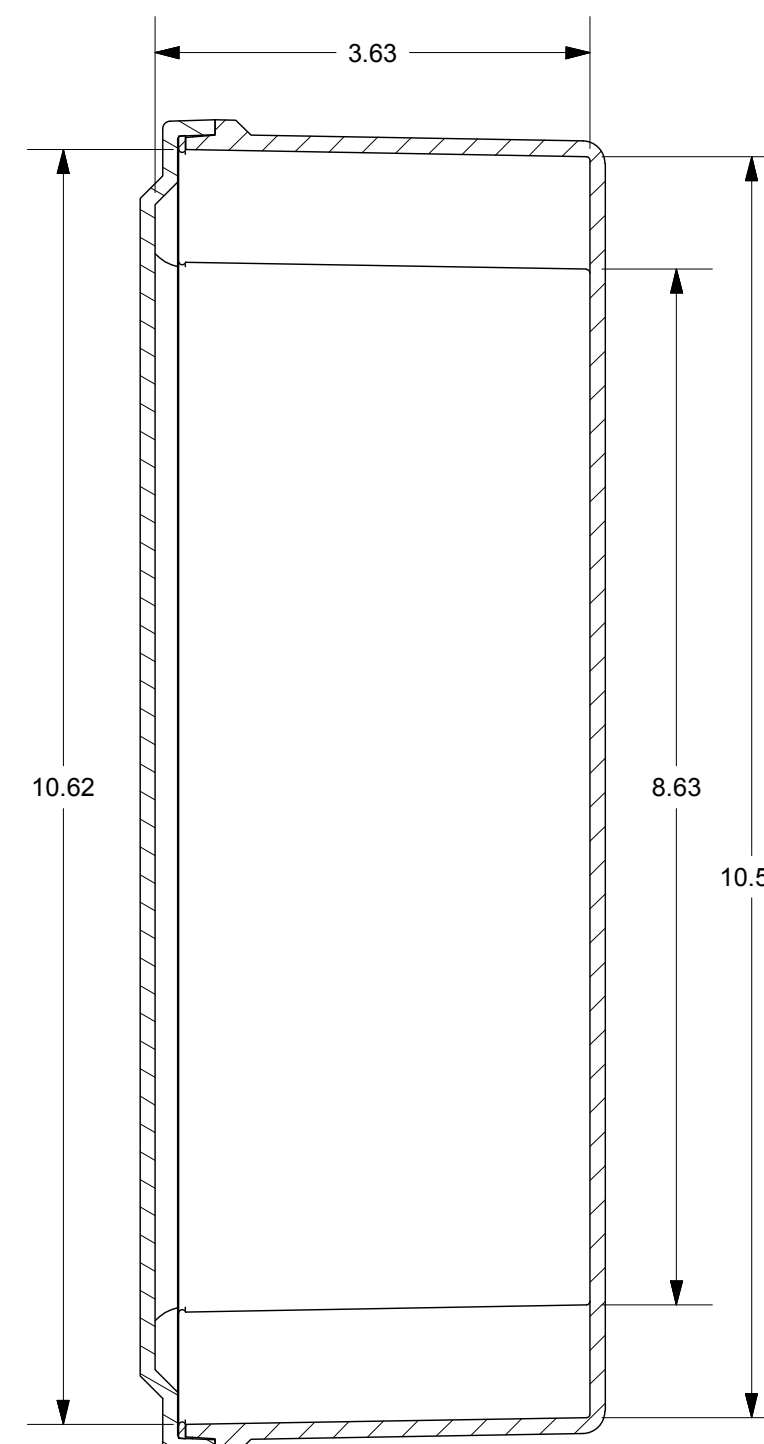
SECTION B-B
