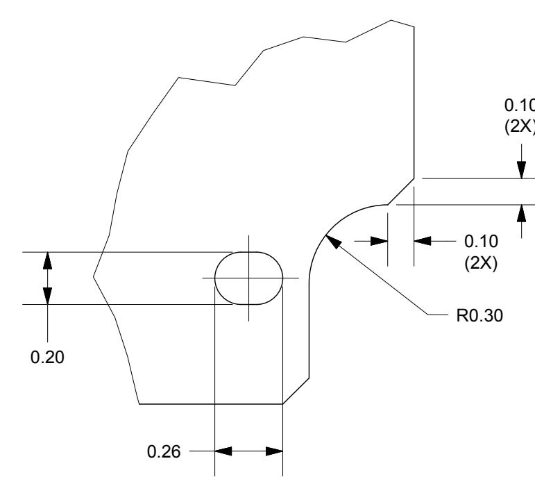
DETAIL A (4X)
