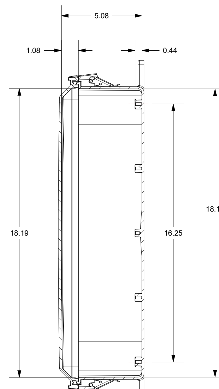
SECTION B-B
